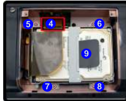
Figure 6 - 3 Hard Disk Assembly Screws & Removal
